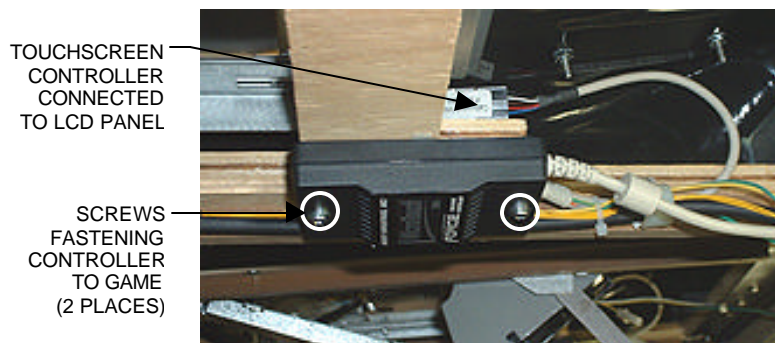
FIGURE 6 - FUSION WITHOUT ELECTRONICS BOX - TOUCHSCREEN CONTROLLER MOUNTED ON BEZEL
