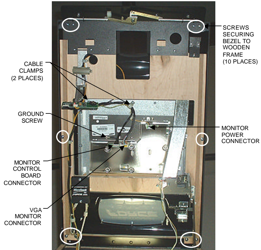
FIGURE 5 - FUSION WITHOUT ELECTRONICS BOX - UNDERSIDE OF BEZEL
