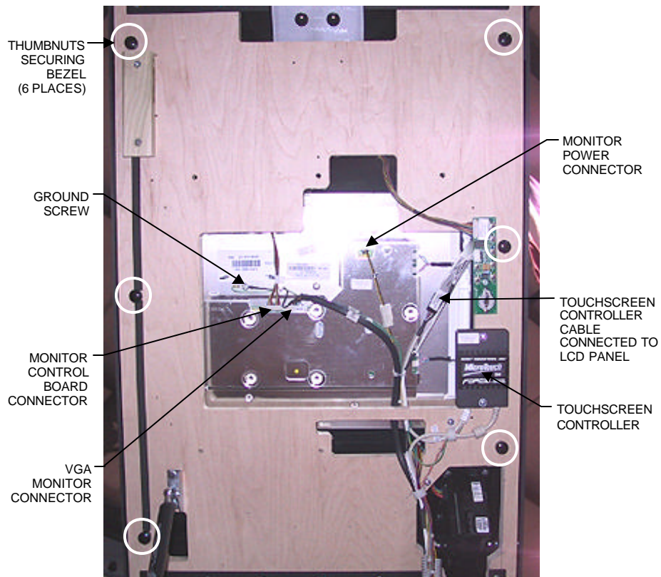
FIGURE 3 - FUSION WITH ELECTRONICS BOX - UNDERSIDE OF BEZEL
