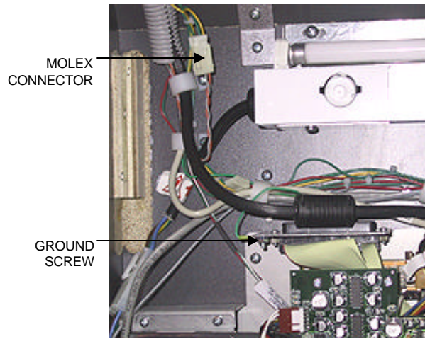
FIGURE 7 - FUSION WITHOUT ELECTRONICS BOX - CLOSEUP OF CPU SECTION
